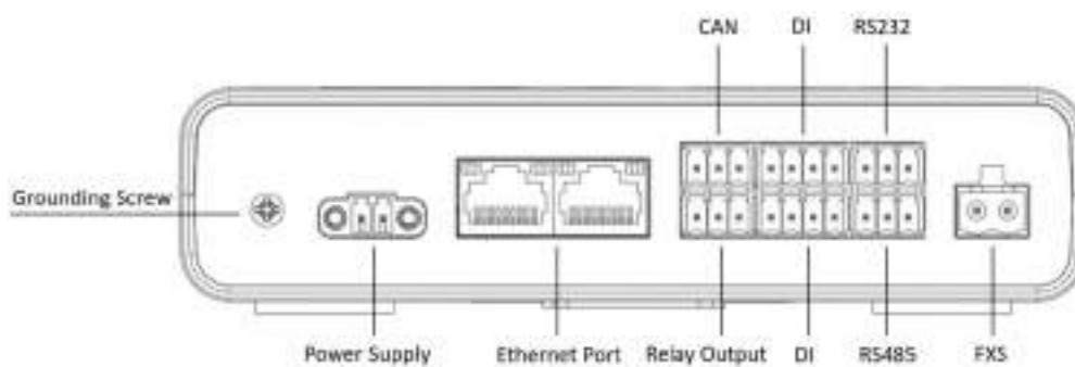
Bottom View
