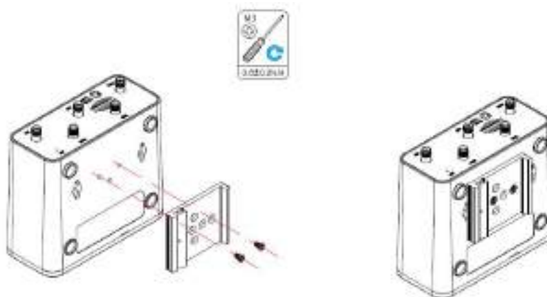
Horizontal installation
