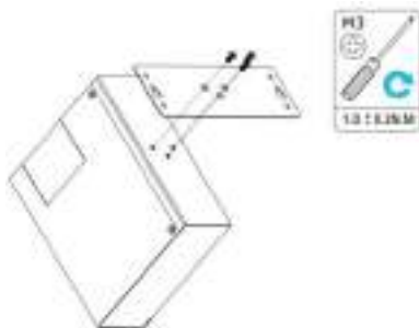
Wall mounting
