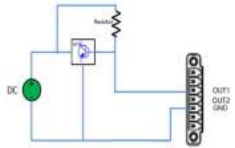
DO connect to NPN transistor(OUT1 for example)
