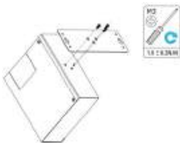
Wall mounting
