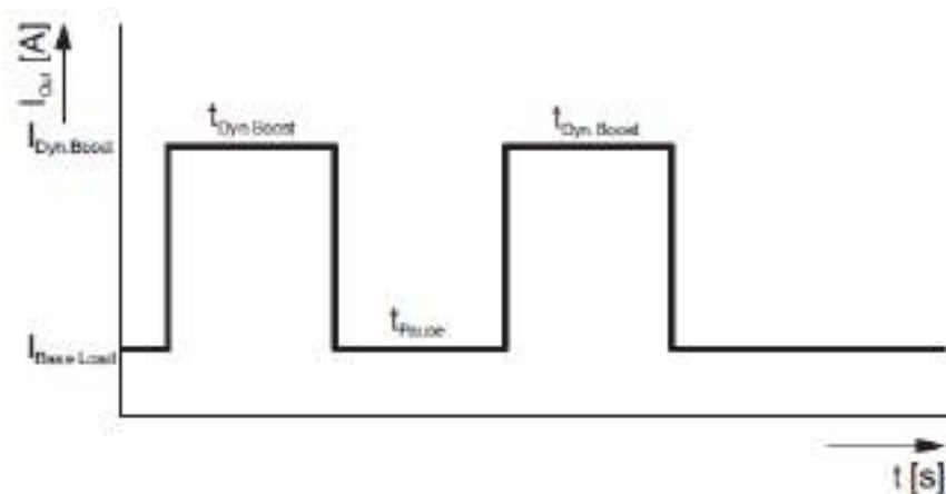
Figure 17 Basic curve of the dynamic boost process
