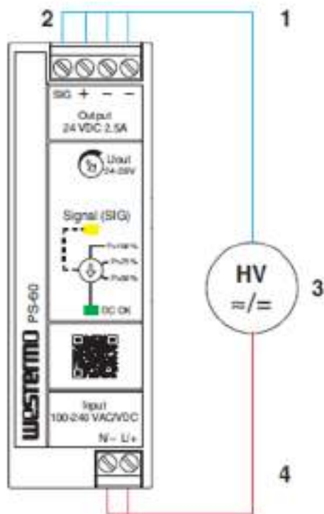
Figure 1 Potential-related wiring for the high-voltage test
