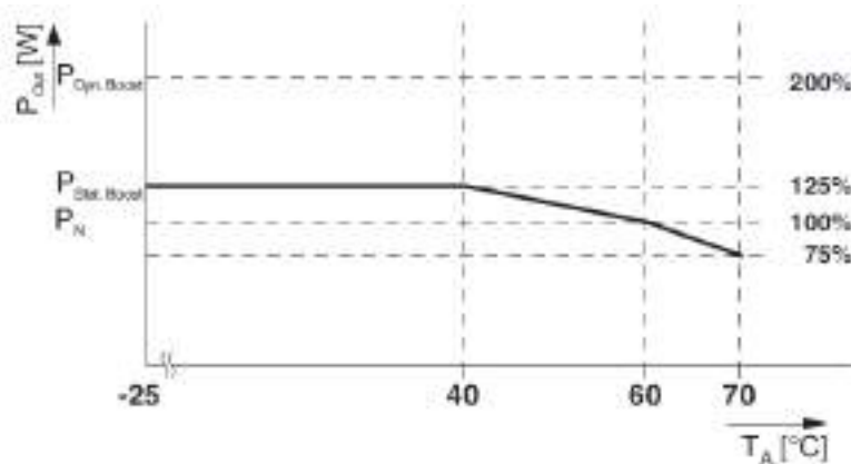
Figure 26 Output power depending on the ambient temperature
