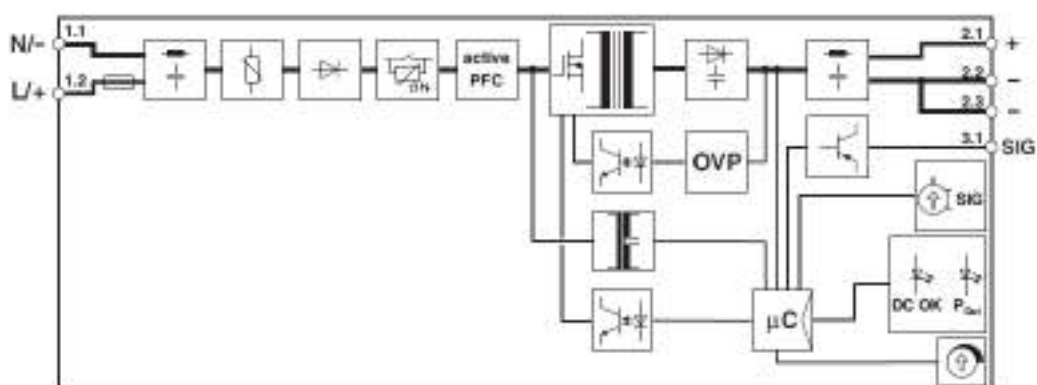
Figure 6 Block diagram
