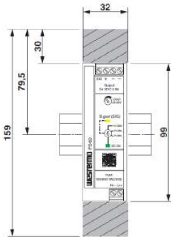
Figure 5 Device dimensions and minimum keep-out areas (in mm)
