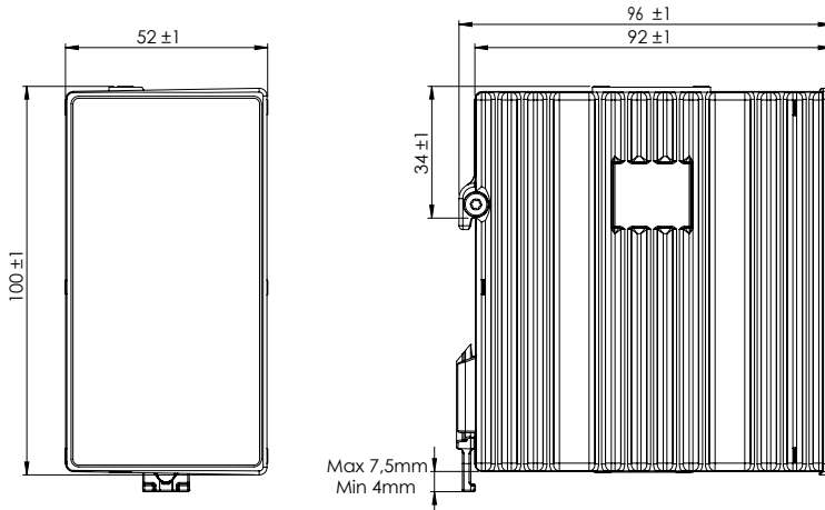
Figure 6. Dimensional drawing
