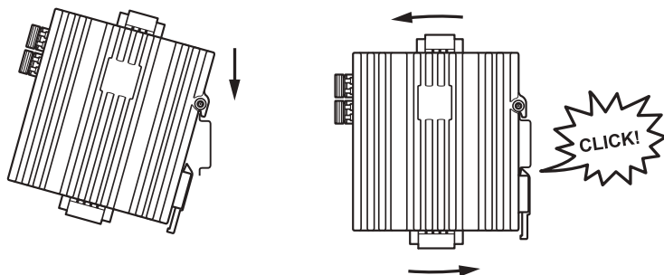
Figure 7. Mounting of product
