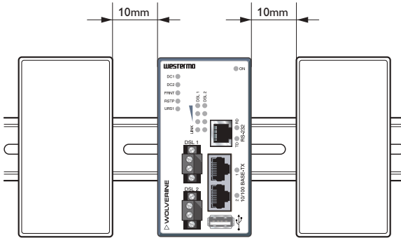
Figure 9. Minimum spacing of product
