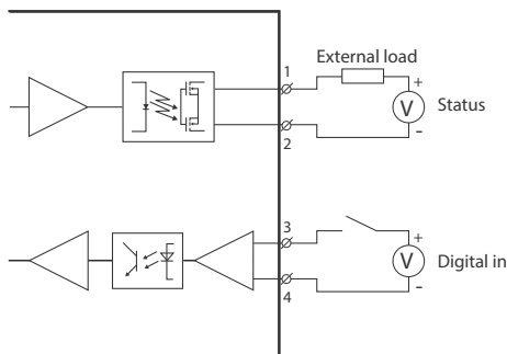
Figure 5. Digital in
