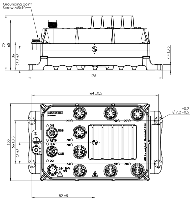
Figure 4. Dimensional drawing
