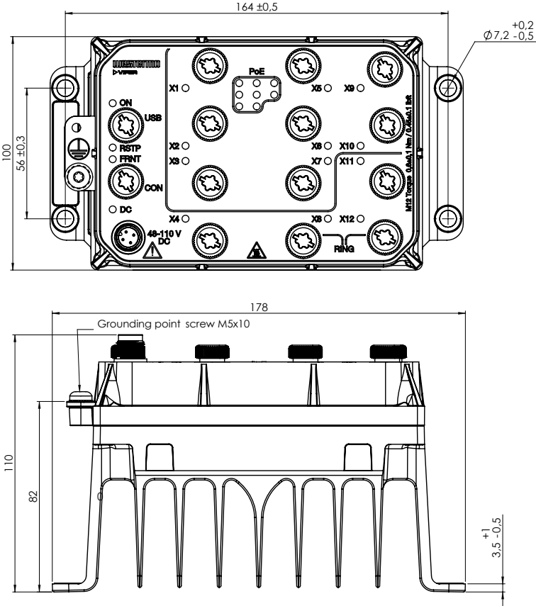
Figure 4. Dimensional drawing
