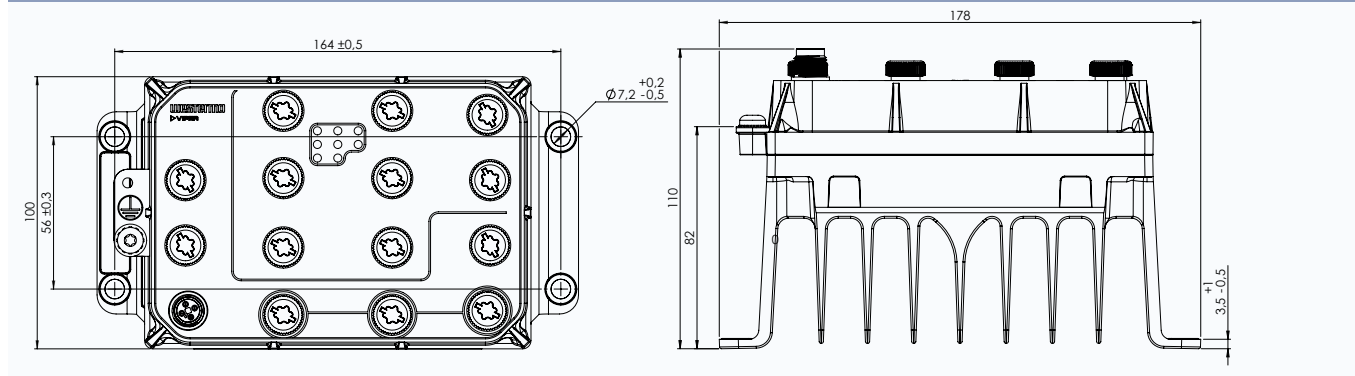
Dimensional drawing
