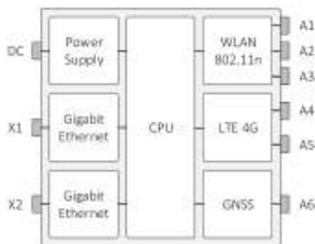
Figure 3. Ibex-RT-630-LV/Ibex-RT-630-HV block diagram
