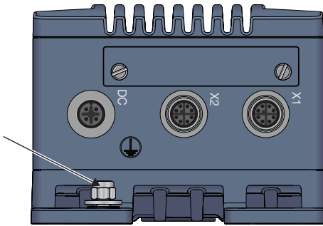
Figure 7. Earth connection
