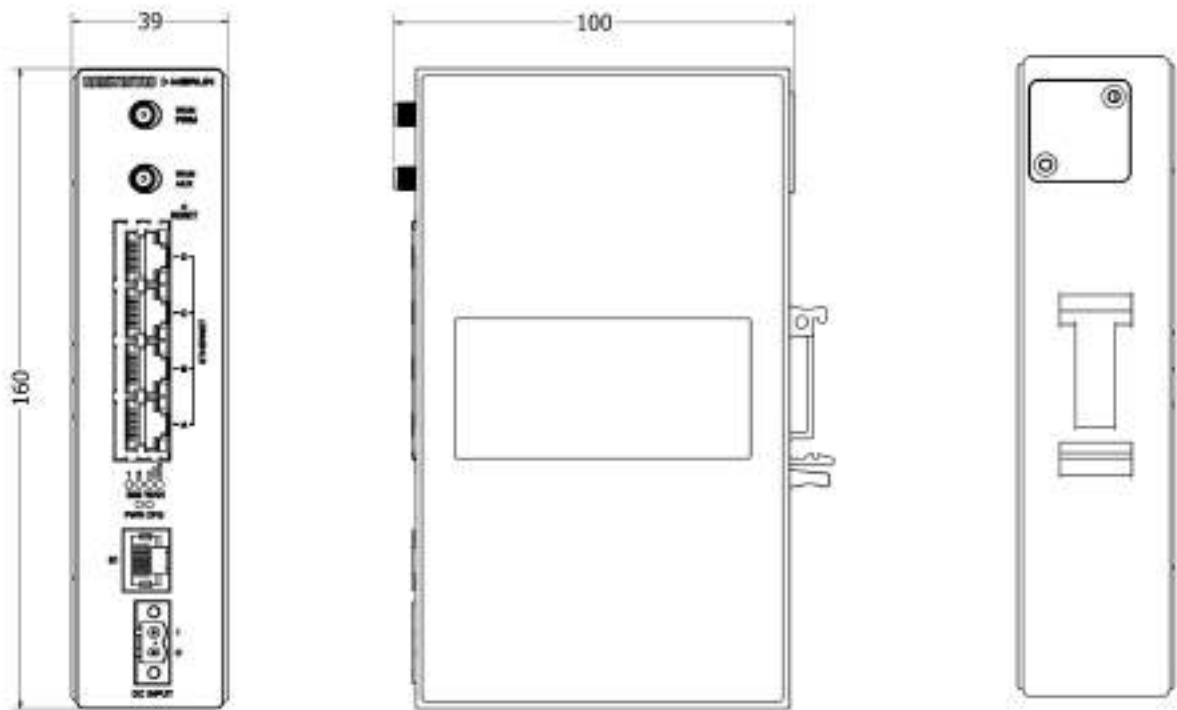
Figure 6. Dimensional drawing
