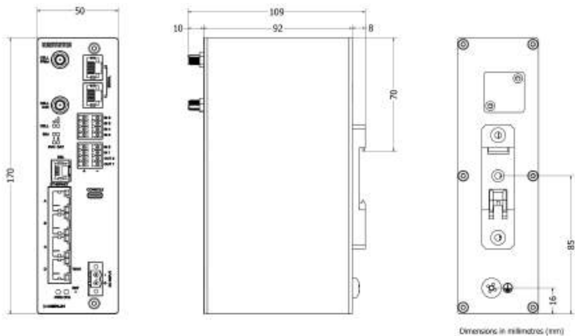
Figure 8. Dimensional drawing
