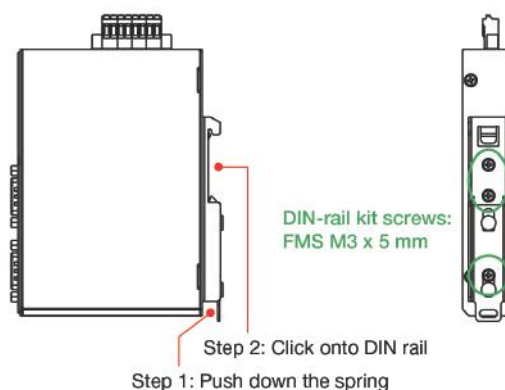
DIN-Rail Installation
